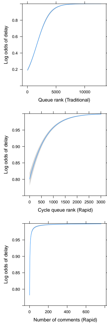
Fig. 14: The relationship between metrics and the release delay . The blue line shows the values of our model fit, whereas the grey area shows the 95% confidence interval based on models fit to 1,000 bootstrap samples. The parentheses indicate the release strategy that the metric is related to.
